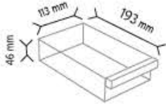
SET120-9 x 9 adet
